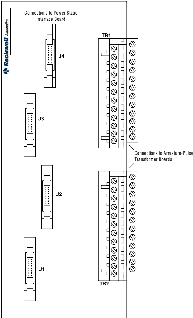
Figure 1.8 Gate Interface Board
